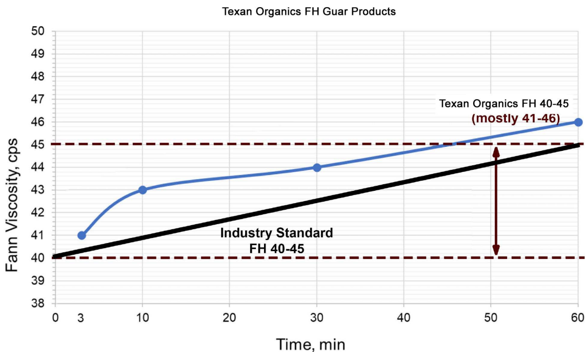
Figure 1. Texan Organics Guar Gum performance in 2% KCL solution at room temperature
